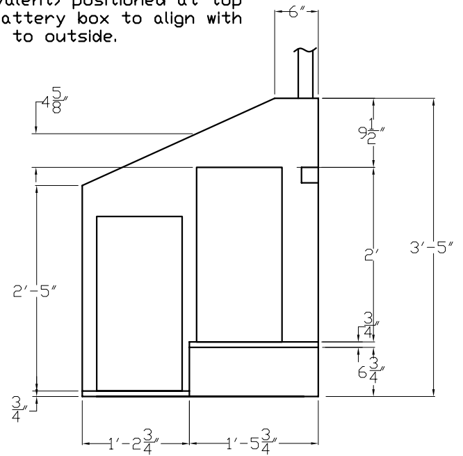
VERT. CROSS-SECTION Overall box dimensions are I.D.
