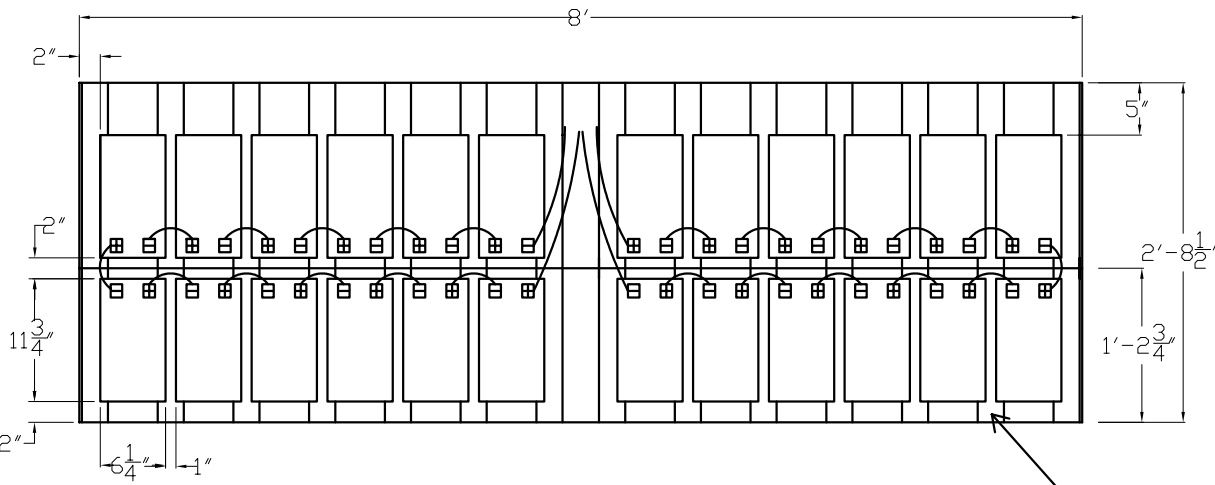
HORIZ. CROSS-SECTION Overall box dimensions are I.D.
